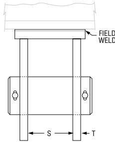
2" Rod Dia. and Larger are Fabricated.
