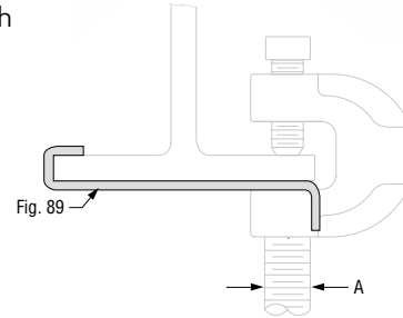
FIG. 89: RETAINING CLIP: WEIGHT (LBS) • DIMENSIONS (IN)
