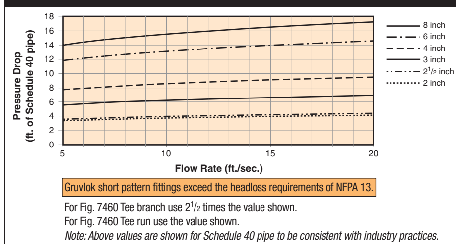
FIGURE 7460 TEE SHORT PATTERN FITTING – PRESSURE DROP
