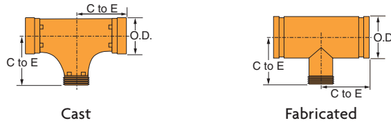
FIGURE 7064 REDUCING TEE WITH THREADED BRANCH
