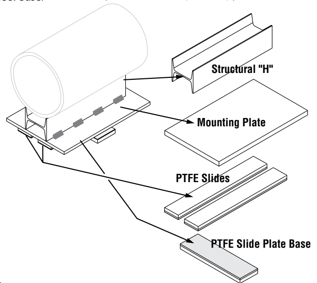
PTFE Pipe Slide Assembly – "H" Type
