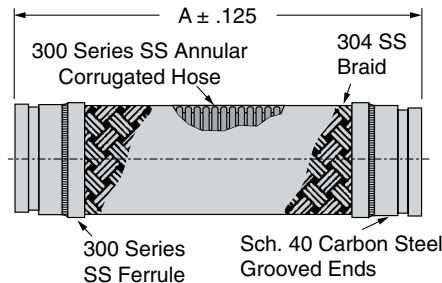
AF-21-GG GRXGR FLEX CONNECTORS
