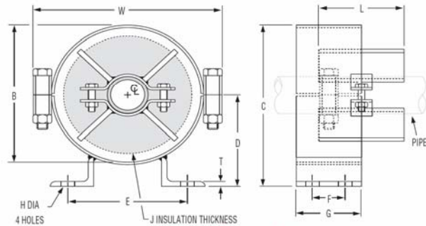
Pipe Alignment Guide Figure 255, Size C Thru J
