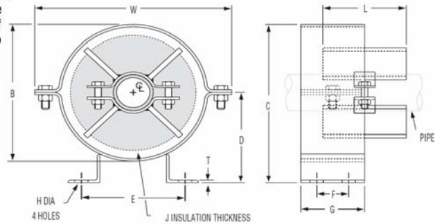
Pipe Alignment Guide Figure 255, Size A&B
